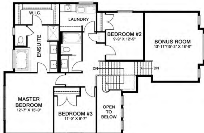
Second Floor Plan 1270 sq. ft.
