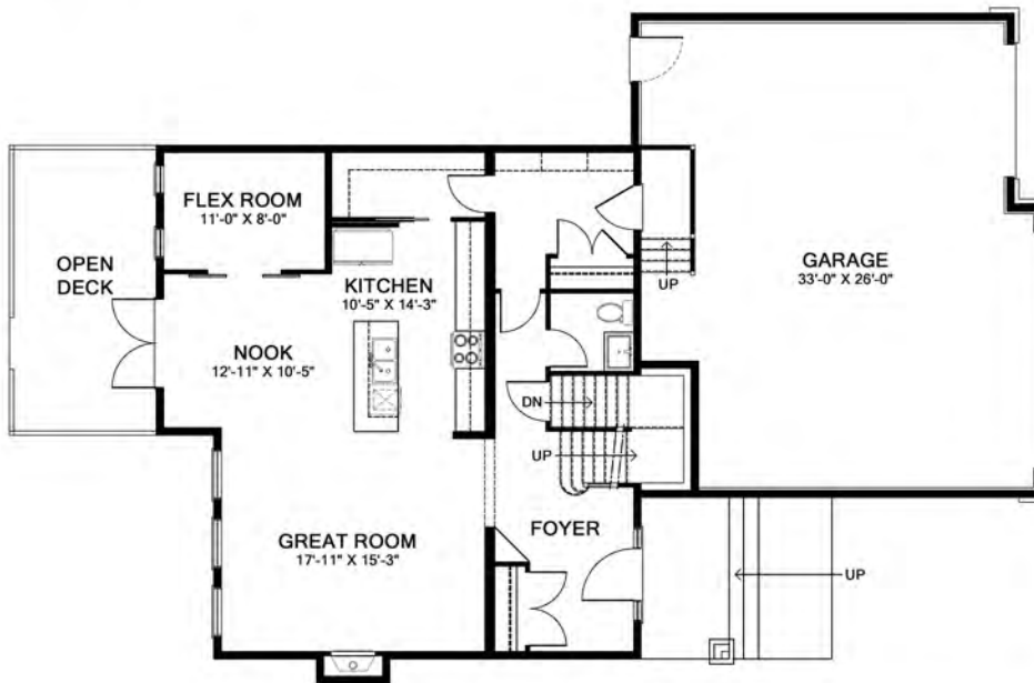
Main Floor Plan 1131 sq. ft.
