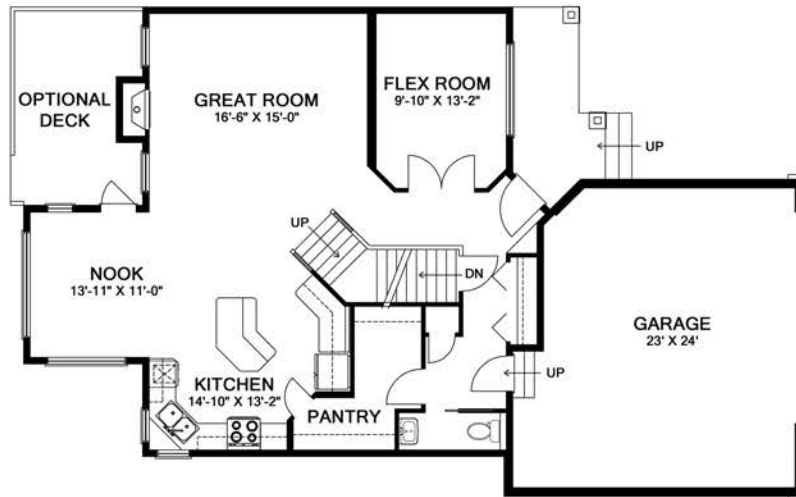
Main Floor Plan 1089 sq. ft.
